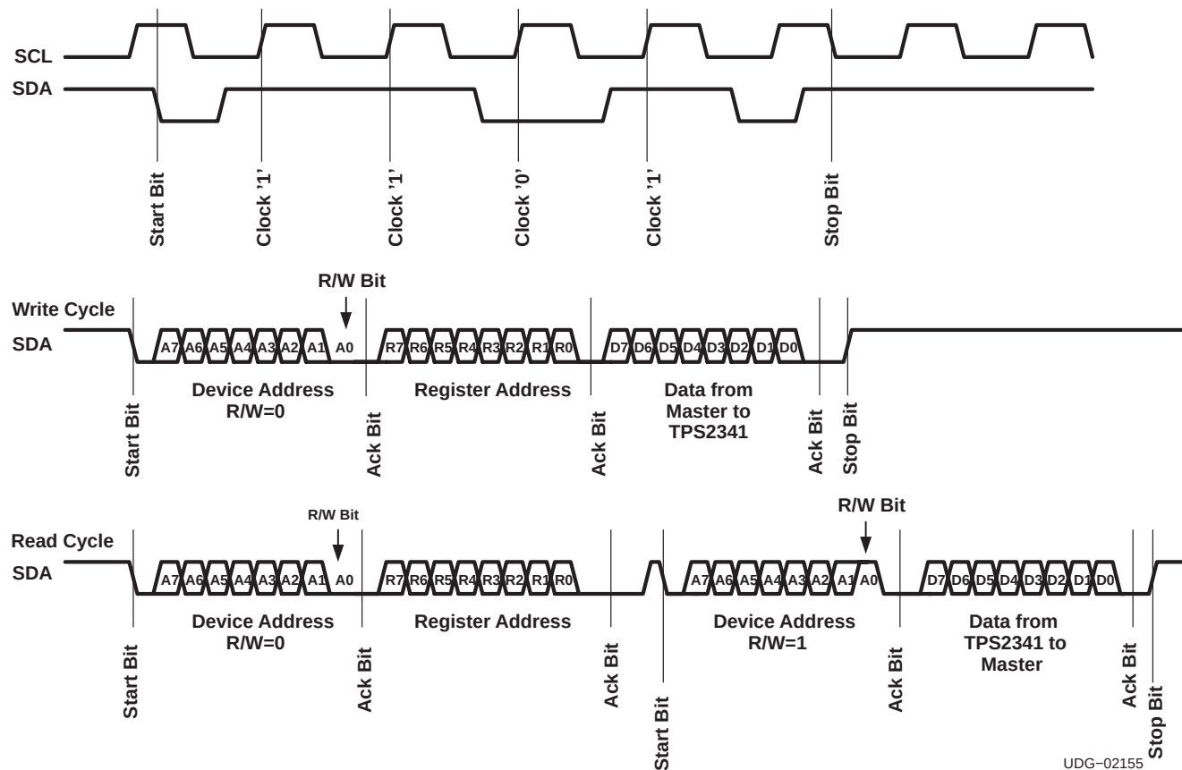
Figure 10. I²C Signal Timing
